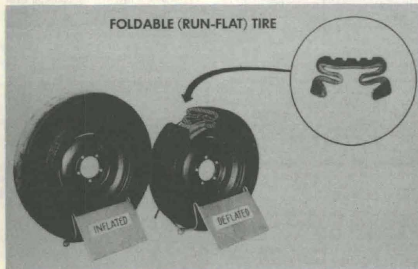
Fig. 2. Foldable run-flat tire and cross section of deflated version.
