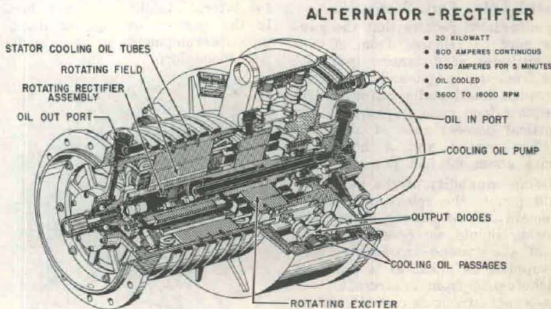
Fig. 2. 20-kw., oil-cooled, electrical generator.
