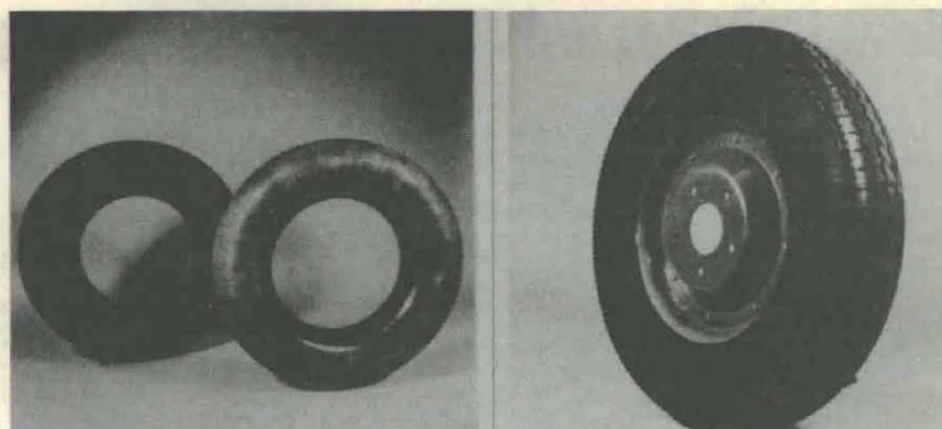
Fig. 3. Filament-wound tire and mounted tire with tread and sidewall rubber.
